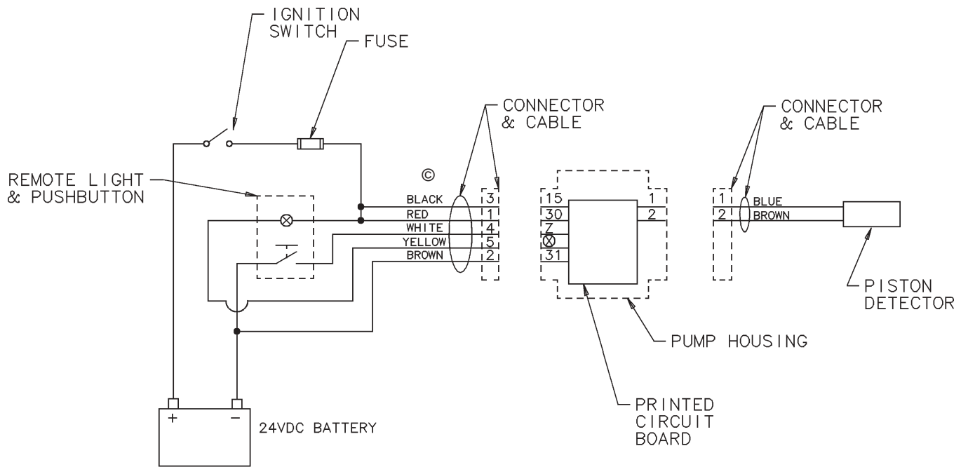
WIRING DIAGRAM FOR POWER AND REMOTE LIGHTED MANUAL LUBE SWITCH
